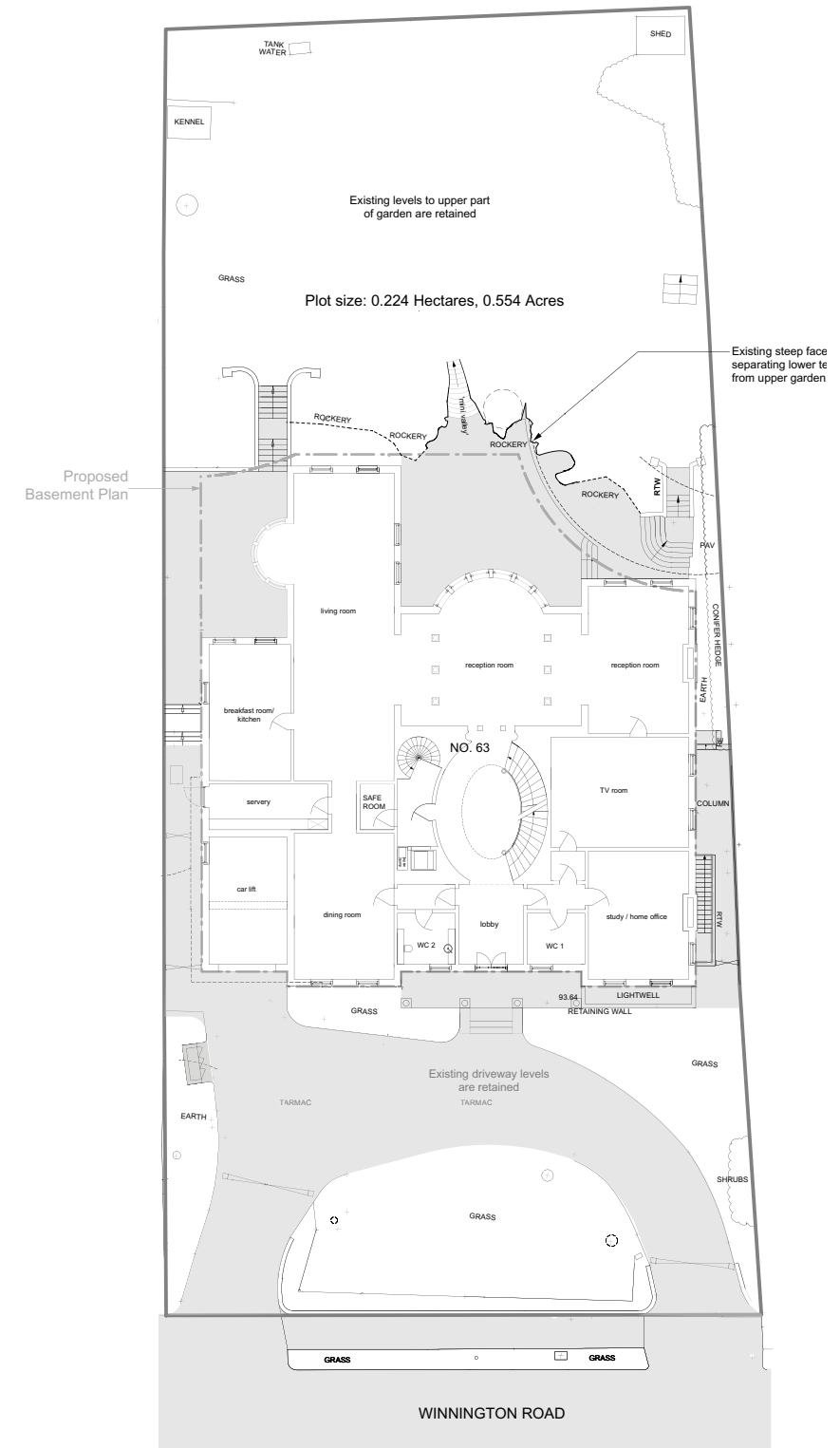
Proposed Site and Ground Floor Plan
