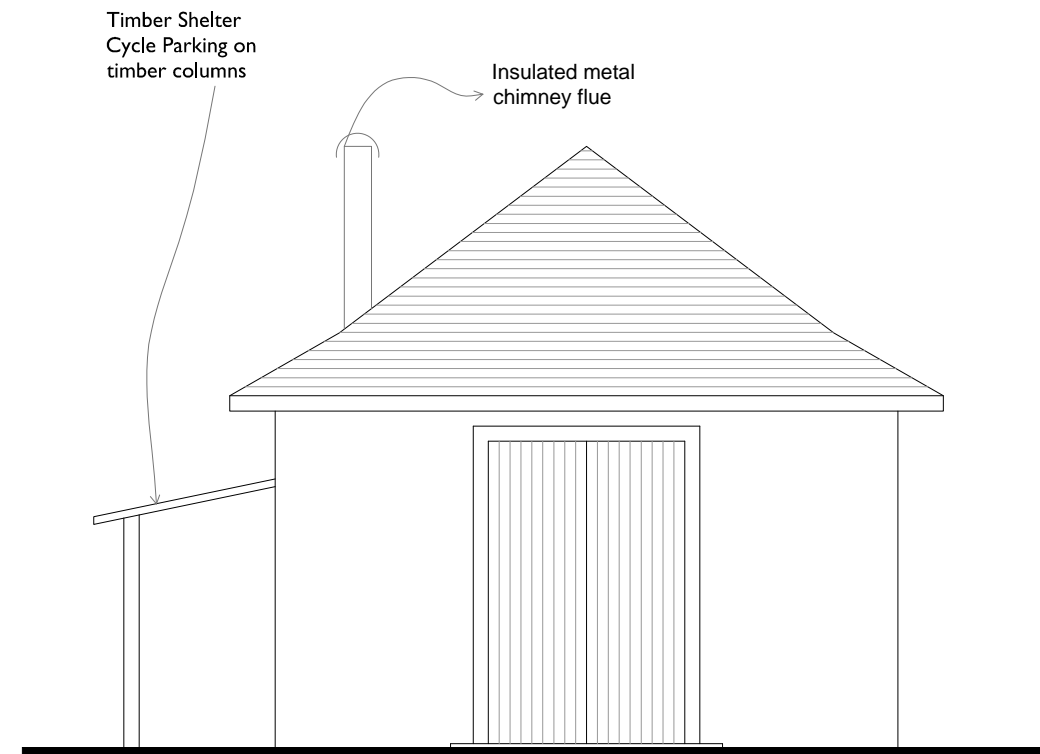
West Elevation
