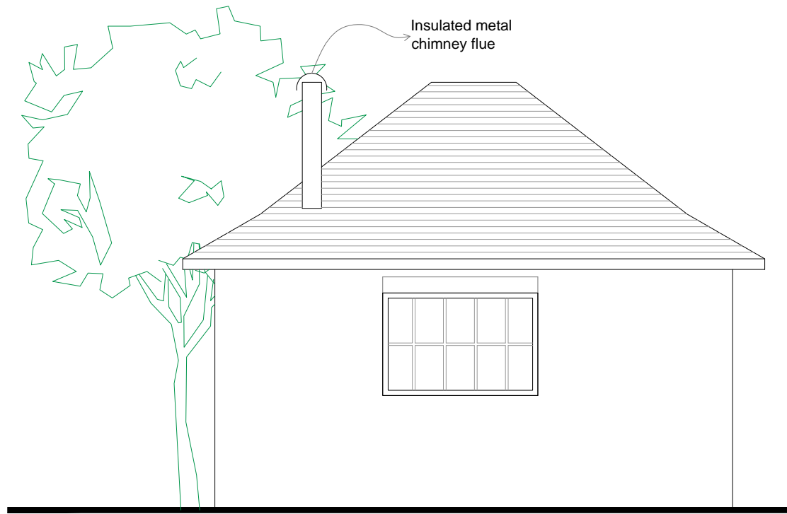
North Elevation
